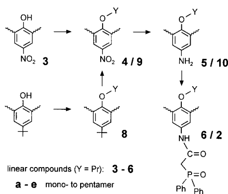
Scheme 1 Synthetic strategies for the preparation of CMPO-calixarenes ( 2 ) and their non cyclic analogs 6 , shown for a single phenolic unit.
