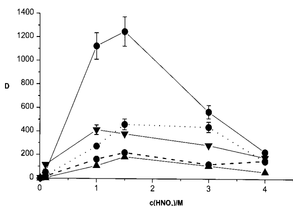
Fig. 2 Distribution coefficient D as function of c(\text{HNO}_3) for the extraction of different cations (Am 3+ (●), Eu 3+ (▲), La 3+ (▼) o -nitrophenyl hexyl ether to (NPHE) by different ligands ( 2b •••, 2c —, 2f - - -). Estimated errors are indicated by bars only where they are distinctly larger than the symbol.
