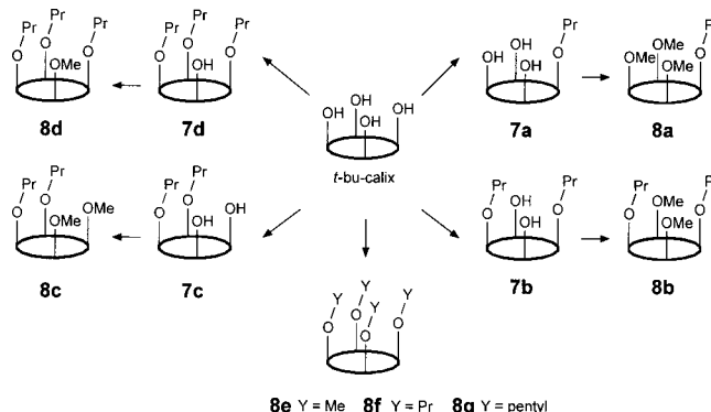
Scheme 2 Synthesis of mixed methyl/propyl ethers 8a–d of t -butyl calix[4]arene and of tetraethers with identical alkoxy groups 8e–g . (The characterization by letters a–g holds also for the subsequent reaction steps 8 → 9 → 10 → 2 , compare Scheme 1.)
