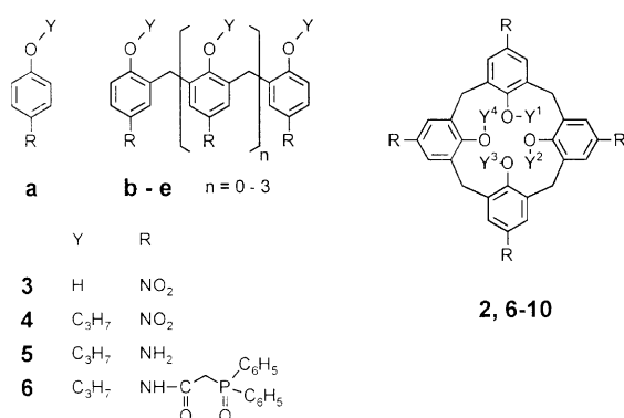
Scheme 1 Synthetic strategies for the preparation of CMPO-calixarenes ( 2 ) and their non cyclic analogs 6 , shown for a single phenolic unit.
